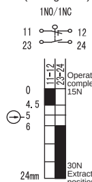
SN6191-SL slow action (Changeover)
