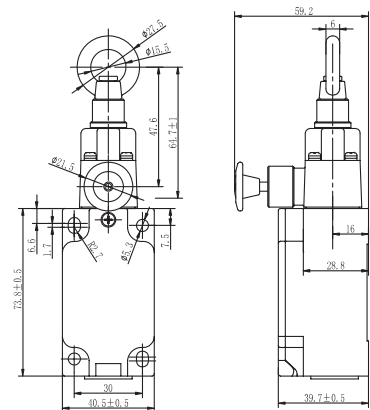
SND6170-SL7-R Slow Action (Overlapping)
