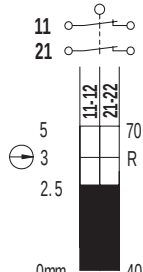
SND6170-SL2-R Slow Action
