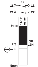
SL2 2NC Slow Action
