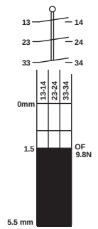
SL5 3NO Slow Action
