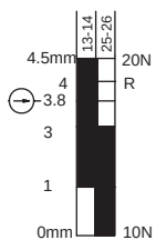
SND4170-SL1-R Slow Action (Overlapping)
