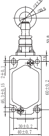
SN6170-SL7 Slow Action (Overlapping)
