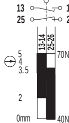
SND6170-SL1 Slow Action (Overlapping)
