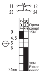
SND4191-SL Slow Action (Changeover) 1NO/1NC
