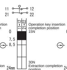
SND4191-SL2 Slow Action 2NC
