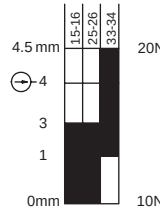
SND2170-SL7 Slow Action (Overlapping)
