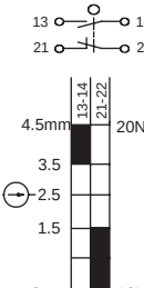
SN4170-SL Slow Action (Changeover)
