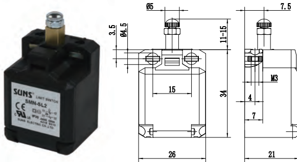
11A Head Style
