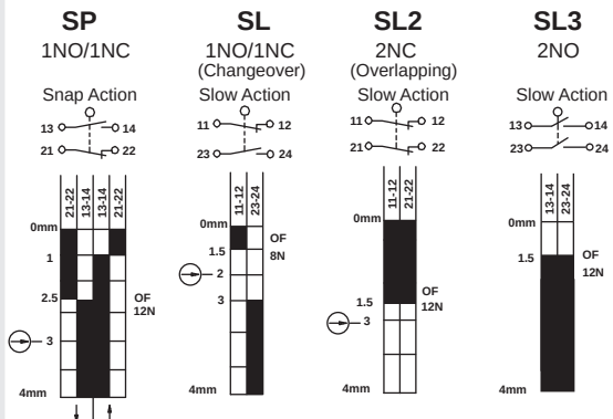
Travel diagrams
