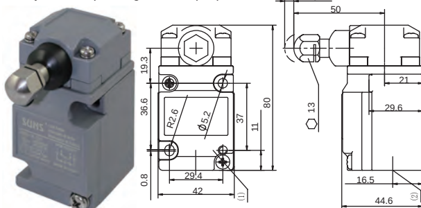
Adjustable Operating Position (OP)
