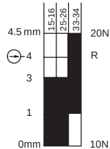
SND4170-SL7-R Slow Action (Overlapping)
