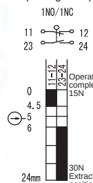
SN6291-SL slow action (Changeover)
