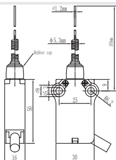
Order Code SM32P11-69 SP snap action 1NO+1NC SM32S11-69 SL slow action 1NO+1NC BBM
